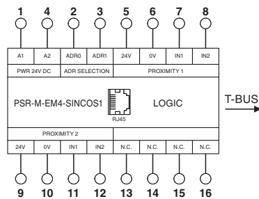
Application drawing
