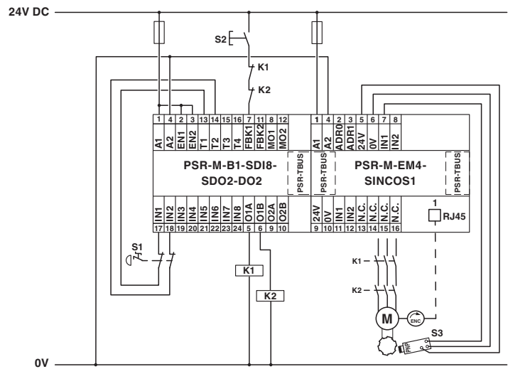
Application drawing
